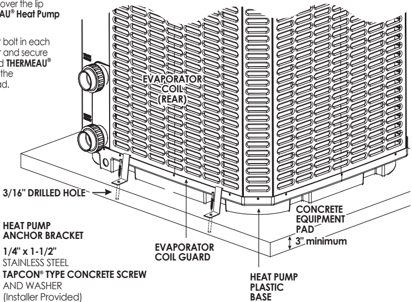
Figure 2. Anchor Clamp Installation
